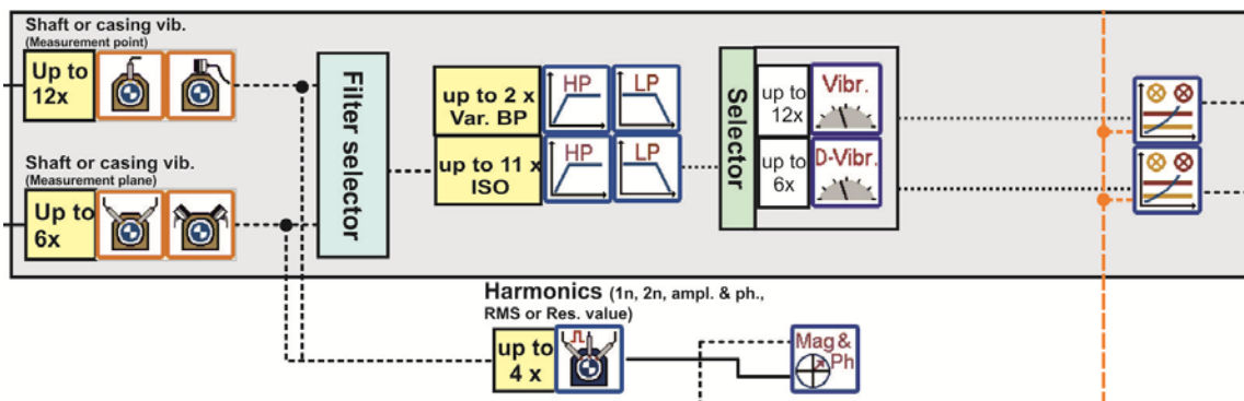
Figure 2: 12 vibration input channels – freely assignable to any input channel with additionally up to 4x Harmonic measurements
